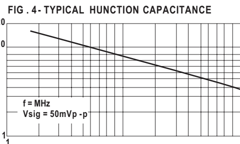
JUNCTION CAPACITANCE (pF)
