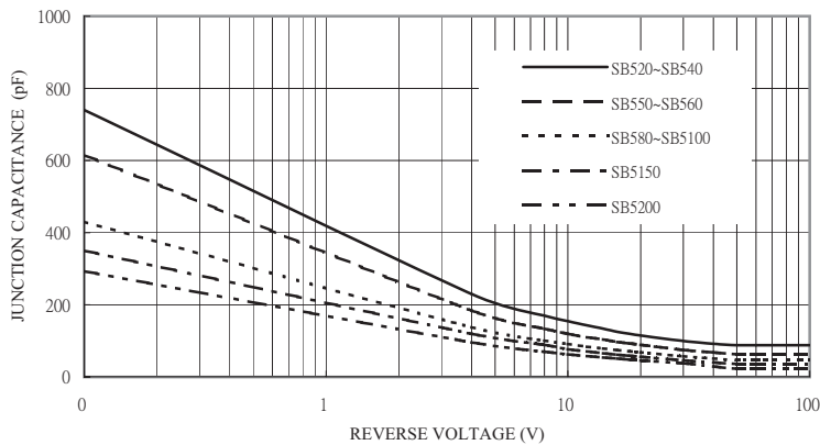
FIG. 4-TYPICAL JUNCTION CAPACITANCE
