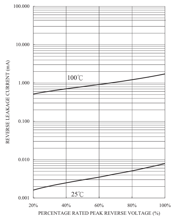
FIG. 5-TYPICAL REVERSE CHARACTERISTICS
