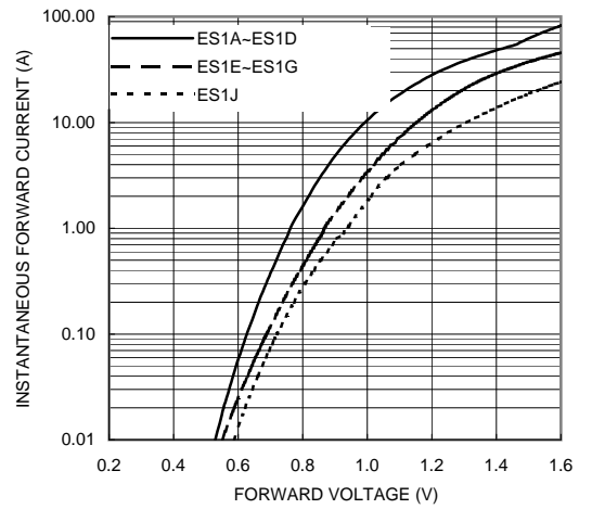
FIG. 2-TYPICAL FORWARD CHARACTERISTICS
