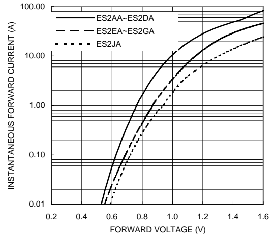
FIG. 2-TYPICAL FORWARD CHARACTERISTICS
