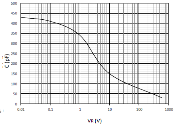
Fig 4. Typical capacitance vs. reverse voltage
