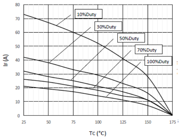
Fig 3. Current Derating
