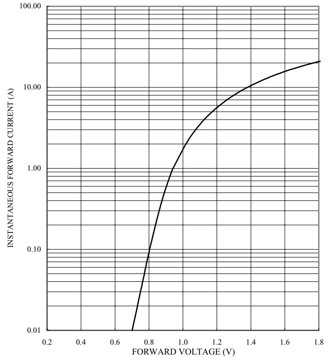
FIG. 2-TYPICAL FORWARD CHARACTERISTICS
